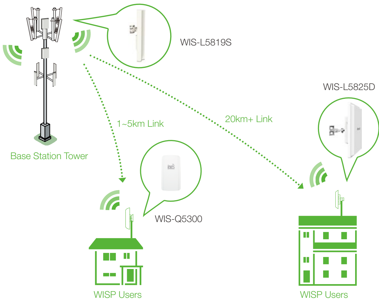
The WIS-L5825D as a station in PtMP WISP connection.
